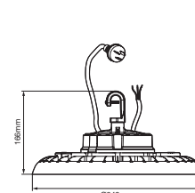
125W/150W/200W Ø343x166mm
