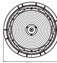
125W/150W/200W Ø343x166mm
