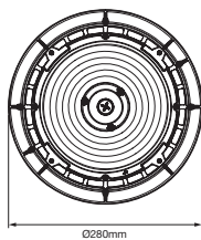
60W/80W/100W Ø280x166mm
