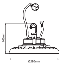
60W/80W/100W Ø280x166mm
